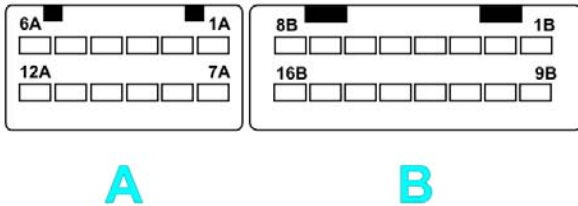
MXL connectors (12 pins “A” and a 16 pins “B” male)
