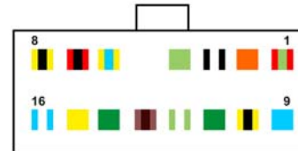
Yamaha 16 pins AMP female connector
